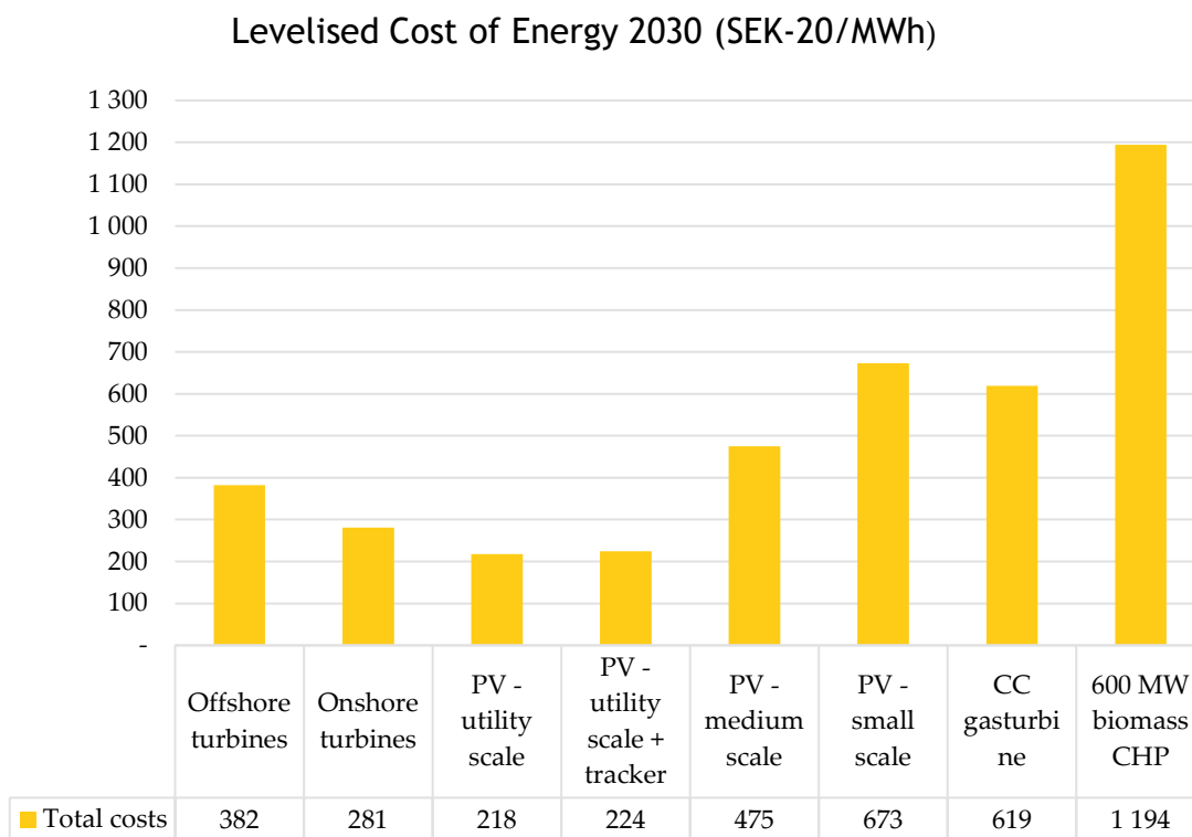
Figure 3: LCOE's for new power generation capacity based on the DEA Technology Catalogue.
