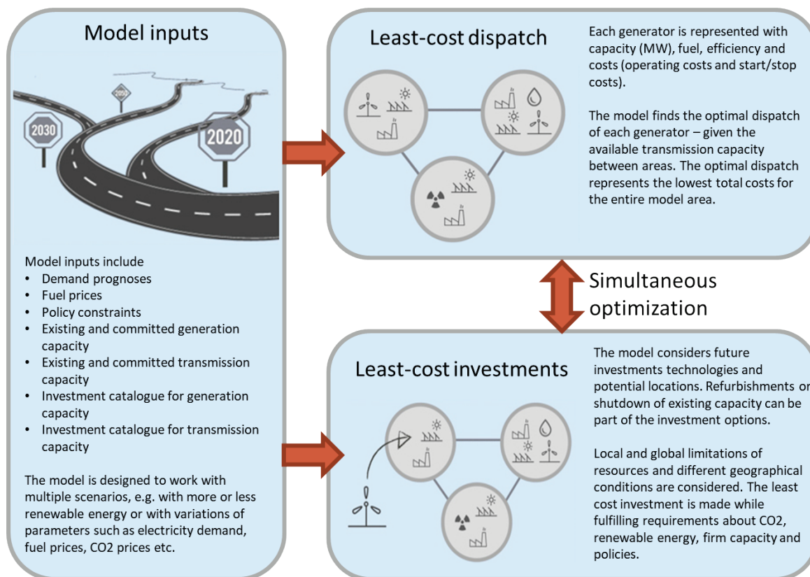
Figure 26. Overview of Balmore model structure.
